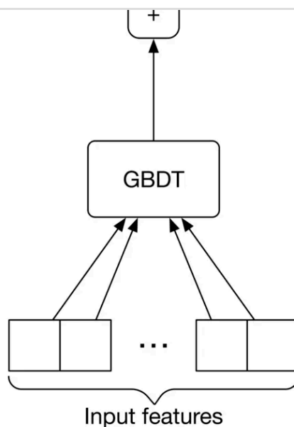
Figure 7.16: A GBDT model with a binary output
