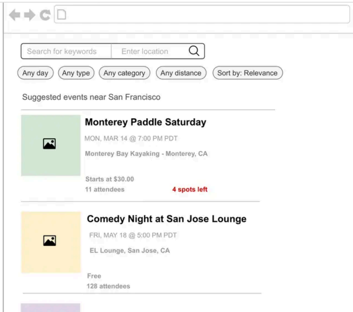
Figure 7.1: Recommended events
