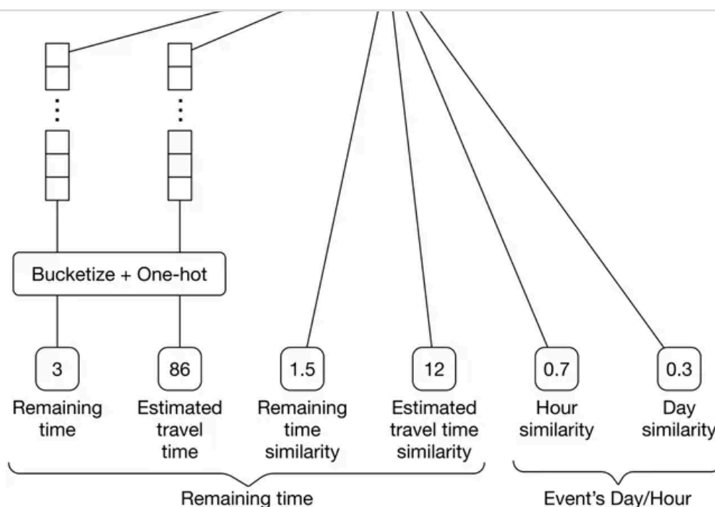
Figure 7.9: Time-related features overview
