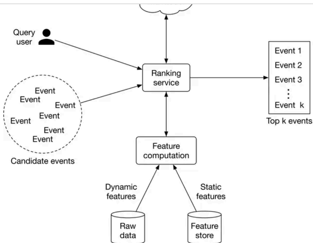
Figure 7.22: Ranking service workflow
