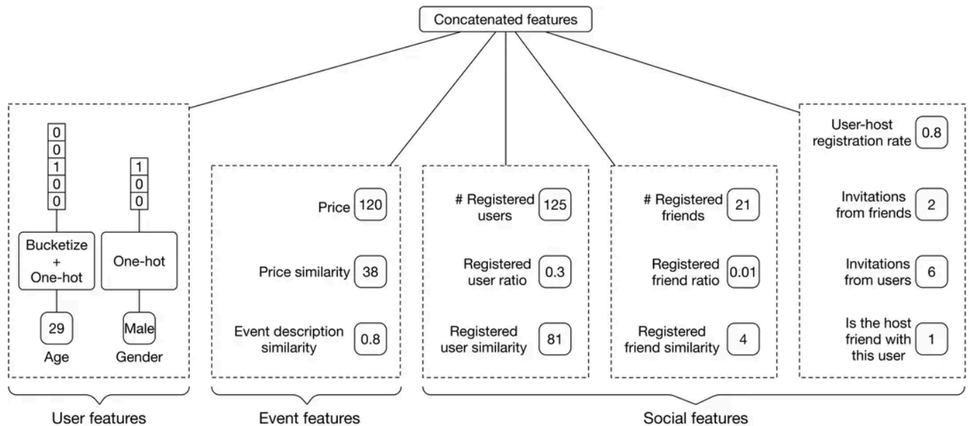
Figure 7.10: User, event, and social features
