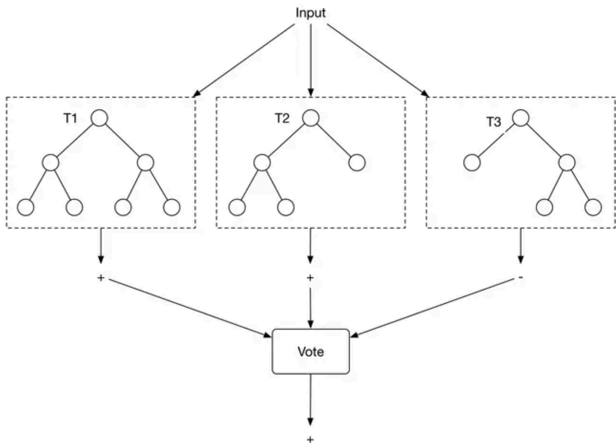
Figure 7.14: Random forest
