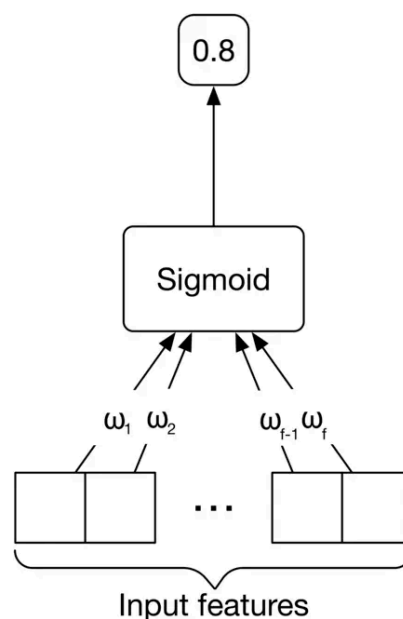
Figure 7.11: Logistic regression
