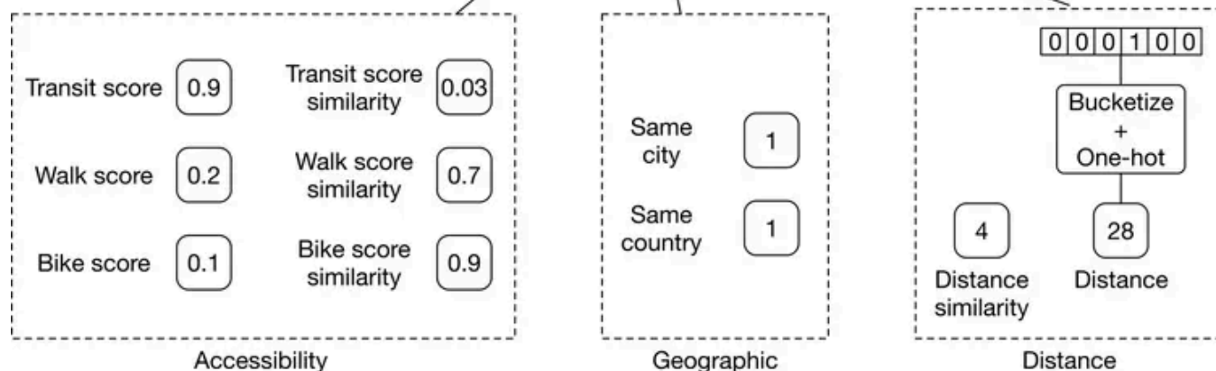
Figure 7.7: Location-related features
